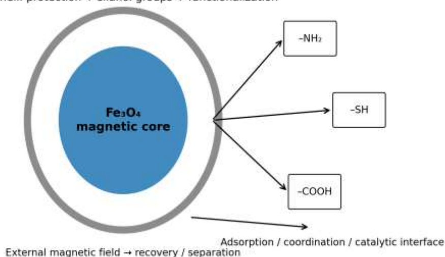
Figure 1. Schematic representation of the Fe 3 O 4 @SiO 2 core-shell platform, showing magnetic core, silica interface and representative functional groups. Original figure prepared for this review.
