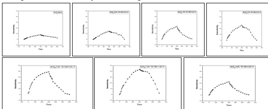
Figure 2 : Gas response of SnO 2 – TX100:F Thin Film for H 2 S.
