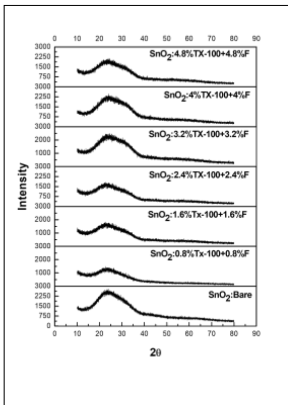
Figure 1: X-ray Diffraction Pattern of SnO 2 with Triton-X100:F Thin Films.
