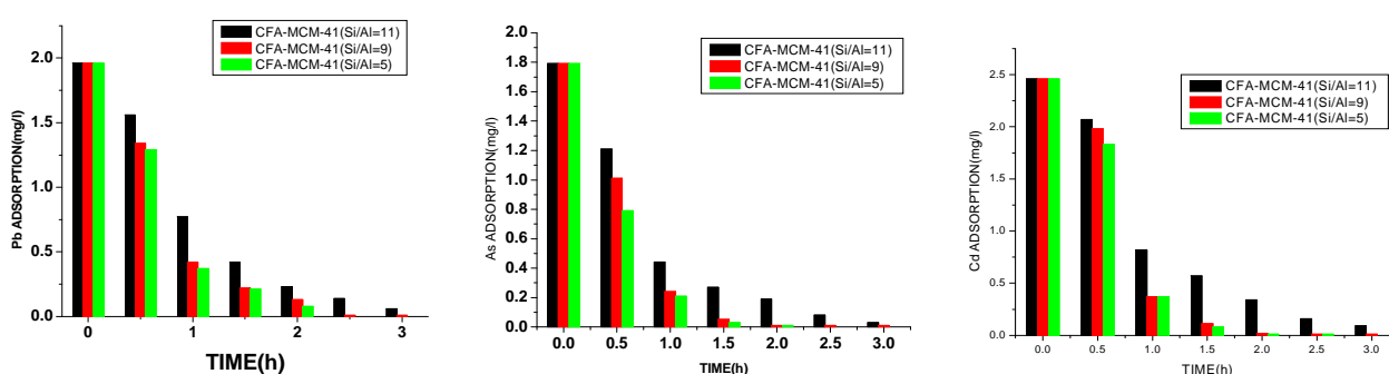
Fig. 5: Variation of the Lead, Arsenic and Cadmium content of Effluent sample with increasing duration of exchange with adsorbents CFA-MCM-41(Si/Al=11, 9 and 5).
