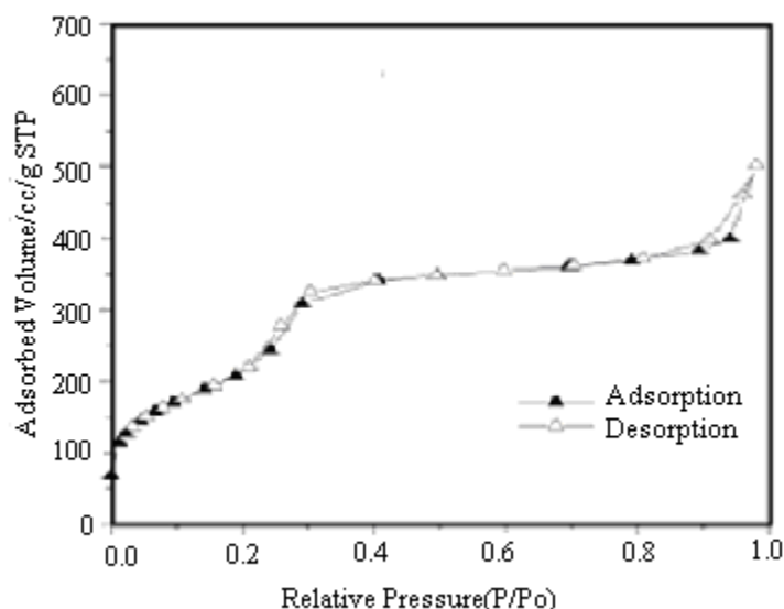
Fig.4: \text{N}_2 -adsorption-desorption isotherms of CFA-MCM-41
