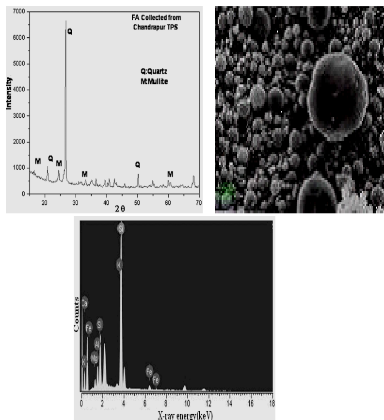
Fig.1 (a)XRD Pattern of treated CFA obtained from Chandrapur TPS (b)The scanning electron micrographs (SEM) of the treated CFA and (c)EDS of CFA
