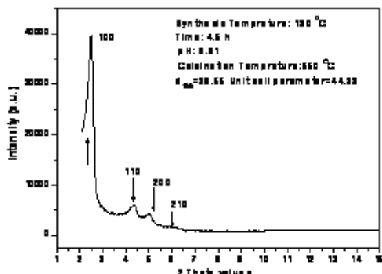
Fig.2: XRD pattern of MCM-41 (100) crystalline at optimized conditions
